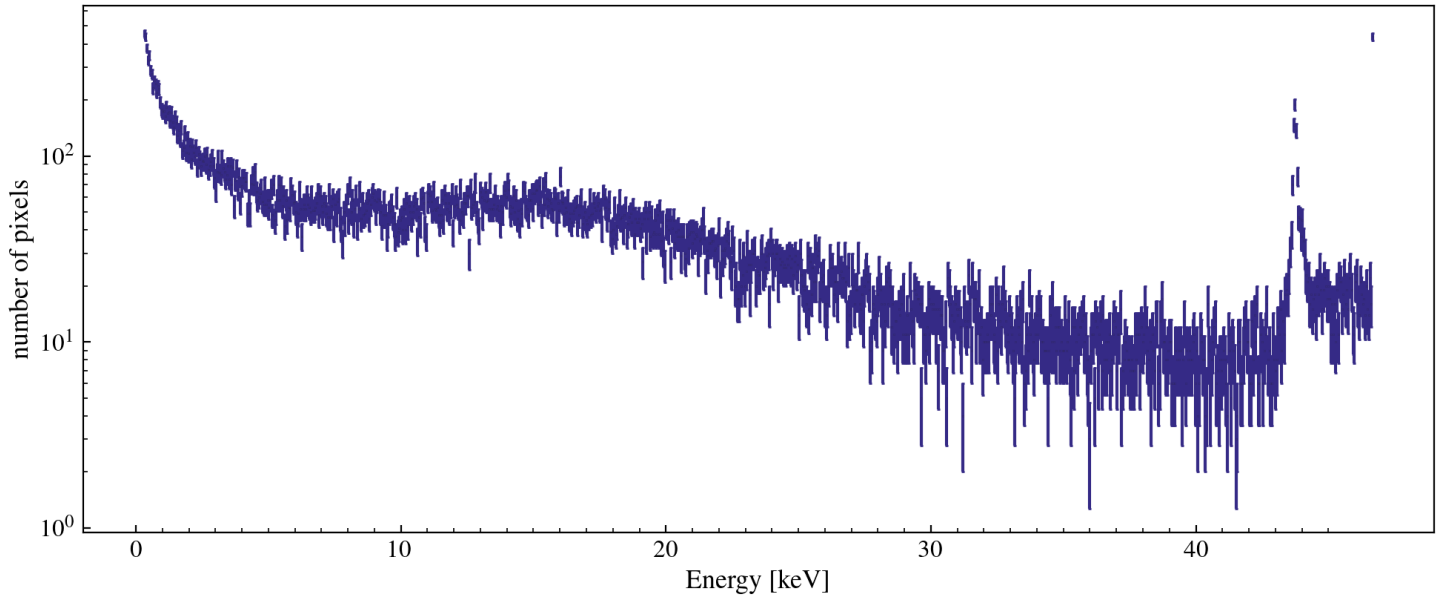
Single Pixel Energy Distribution [w/ 5.16 ADC/e- and 3.74eV/e-] [class MESinglePED]
