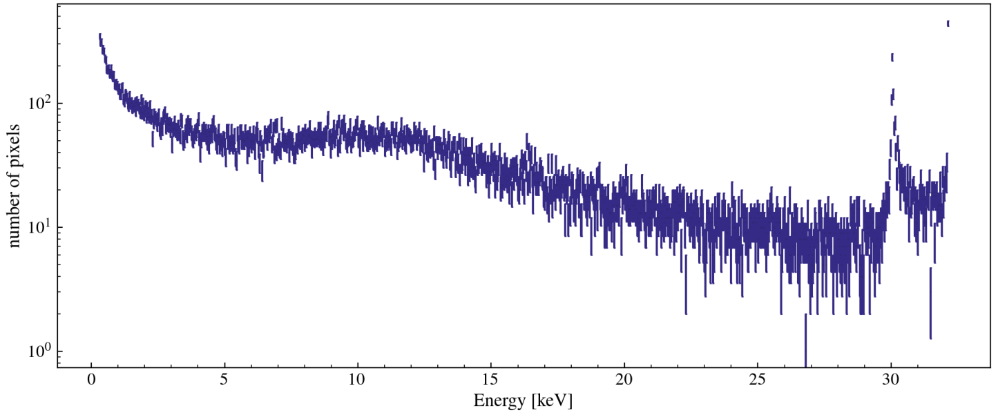
Single Pixel Energy Distribution [w/ 7.5 ADC/e- and 3.74eV/e-] [class MESinglePED]
