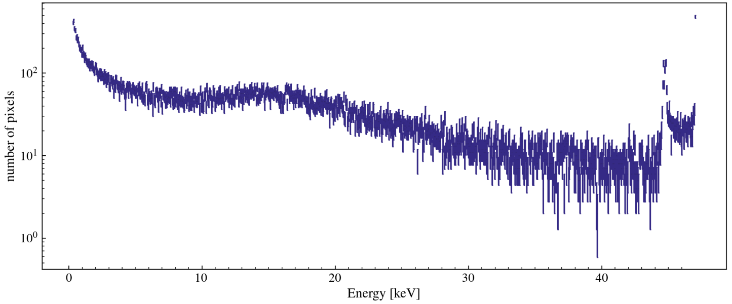
Single Pixel Energy Distribution [w/ 5.12 ADC/e- and 3.74eV/e-] [class MESinglePED]
