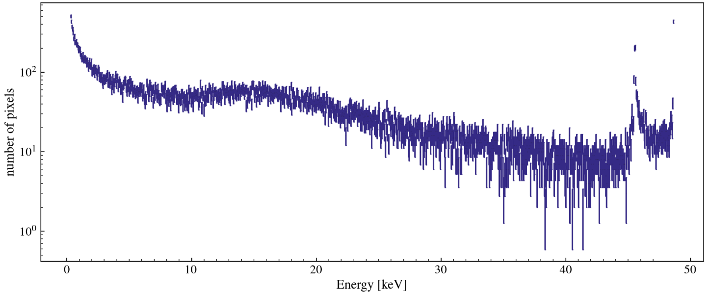
Single Pixel Energy Distribution [w/ 4.96 ADC/e- and 3.74eV/e-] [class MESinglePED]
