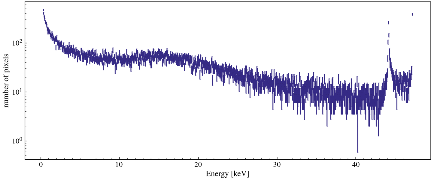
Single Pixel Energy Distribution [w/ 5.11 ADC/e- and 3.74eV/e-] [class MESinglePED]
