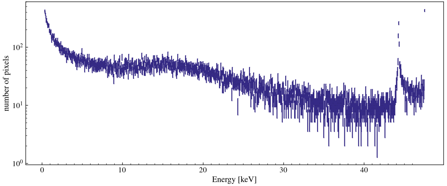
Single Pixel Energy Distribution [w/ 5.07 ADC/e- and 3.74eV/e-] [class MESinglePED]
