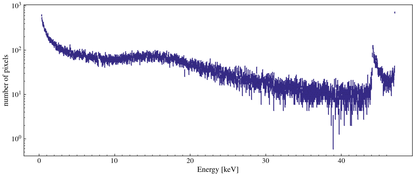
Single Pixel Energy Distribution [w/ 5.12 ADC/e- and 3.74eV/e-] [class MESinglePED]
