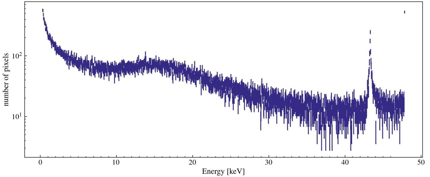
Single Pixel Energy Distribution [w/ 5.04 ADC/e- and 3.74eV/e-] [class MESinglePED]
