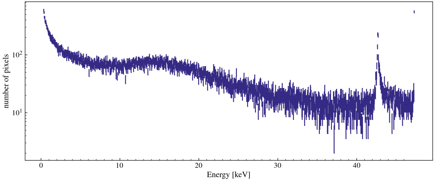
Single Pixel Energy Distribution [w/ 5.09 ADC/e- and 3.74eV/e-] [class MESinglePED]
