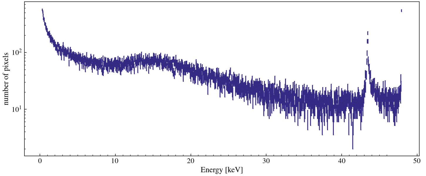
Single Pixel Energy Distribution [w/ 5.03 ADC/e- and 3.74eV/e-] [class MESinglePED]
