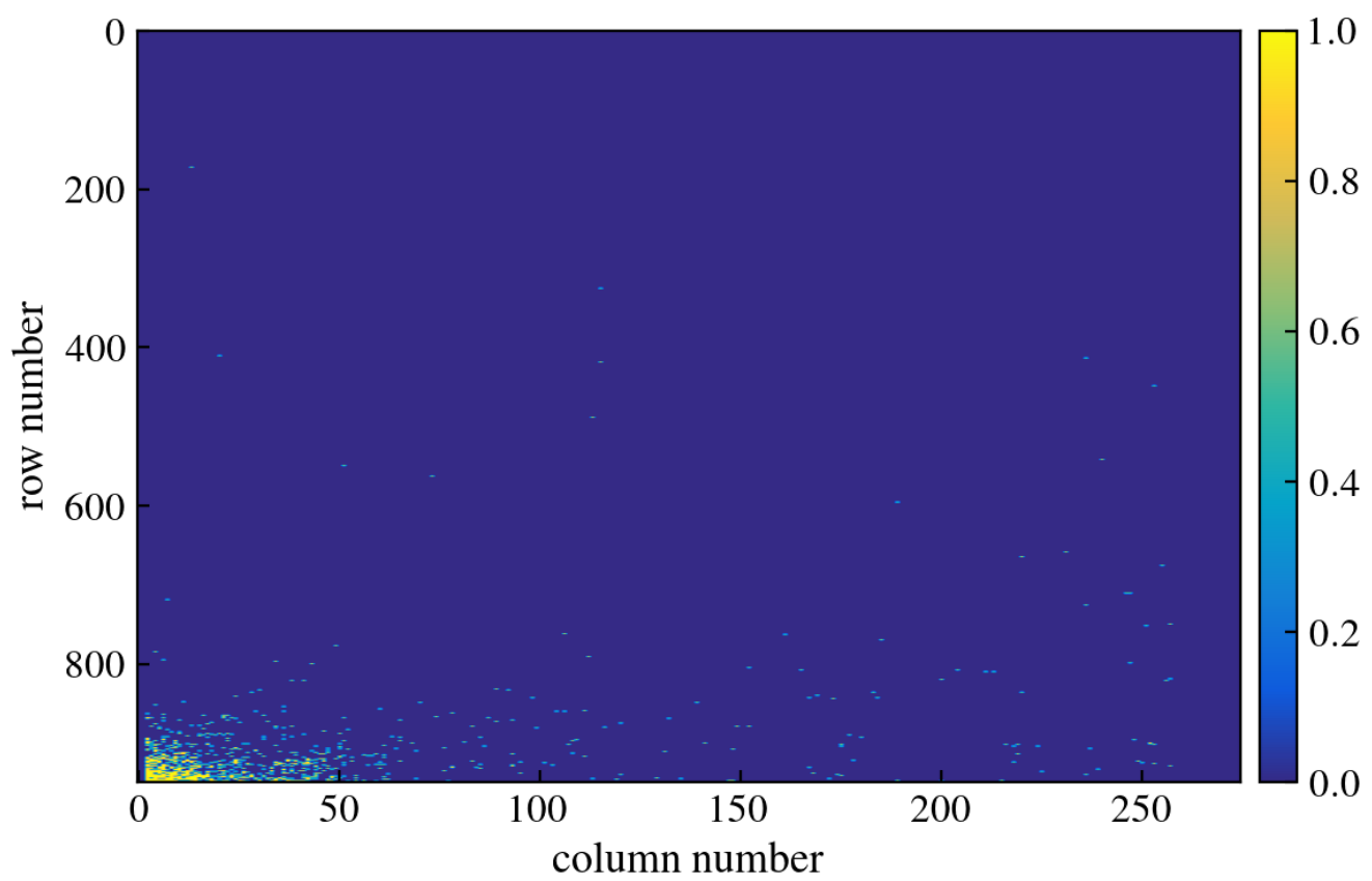
Figure 15: Masked pixels
