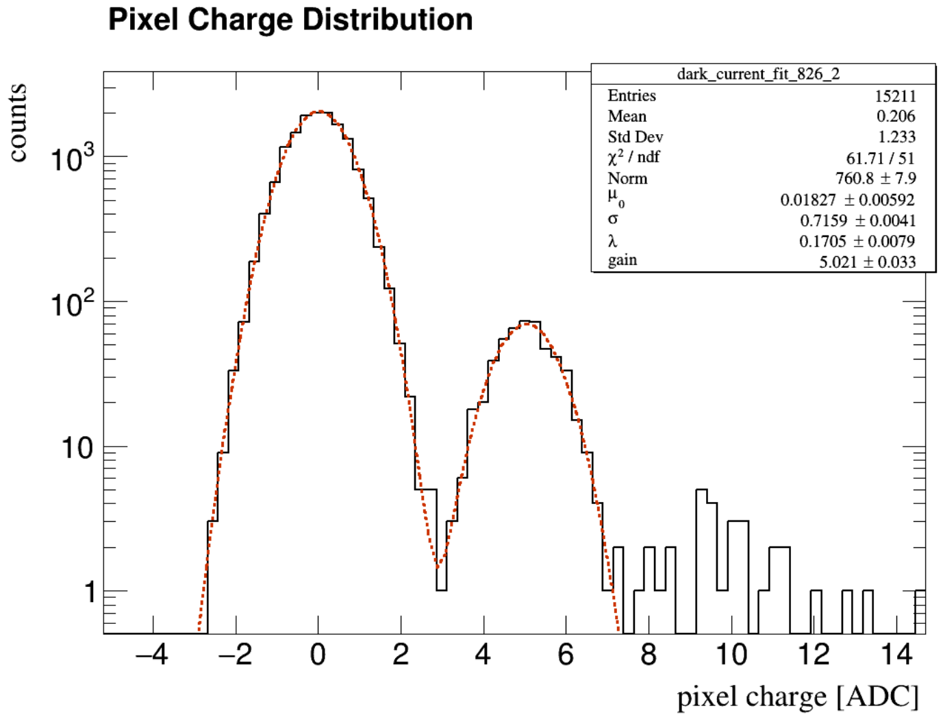
Figure 18: Pixel Charge Distribution
