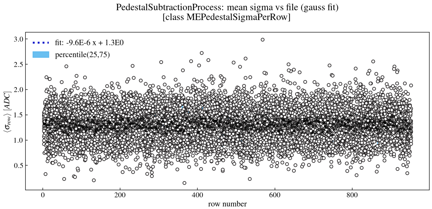
Figure 13: PedestalSubtractionProcess: mean sigma vs file (gauss fit)
