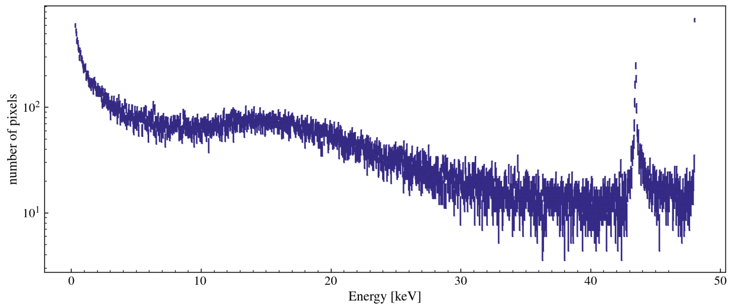
Single Pixel Energy Distribution [w/ 5.02 ADC/e- and 3.74eV/e-] [class MESinglePED]
