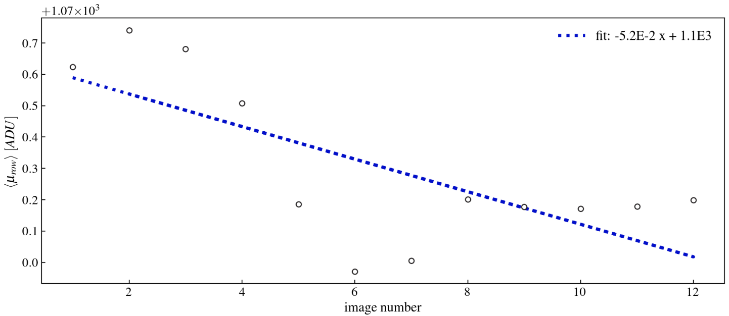
Figure 10: PedestalSubtractionProcess: mean pedestal vs file (gauss fit)
