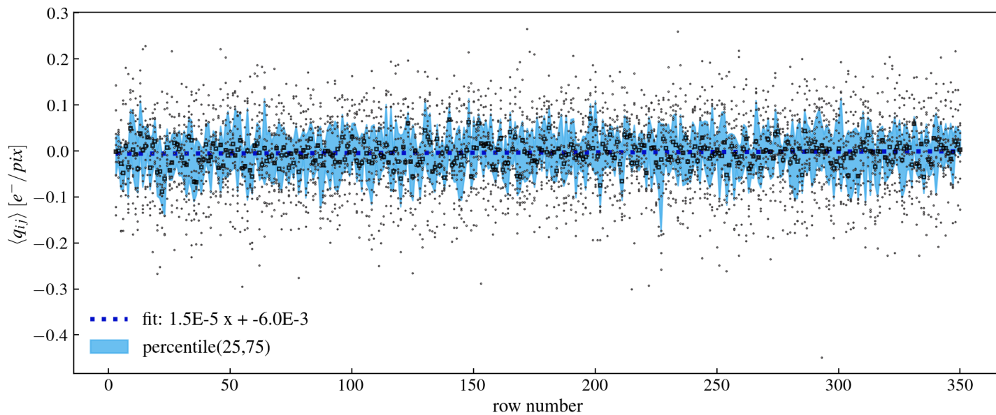
Active Area. Median dark current (only q_{i,j} < q_i^{th} ) vs row [class MEMeanDCperRow]
