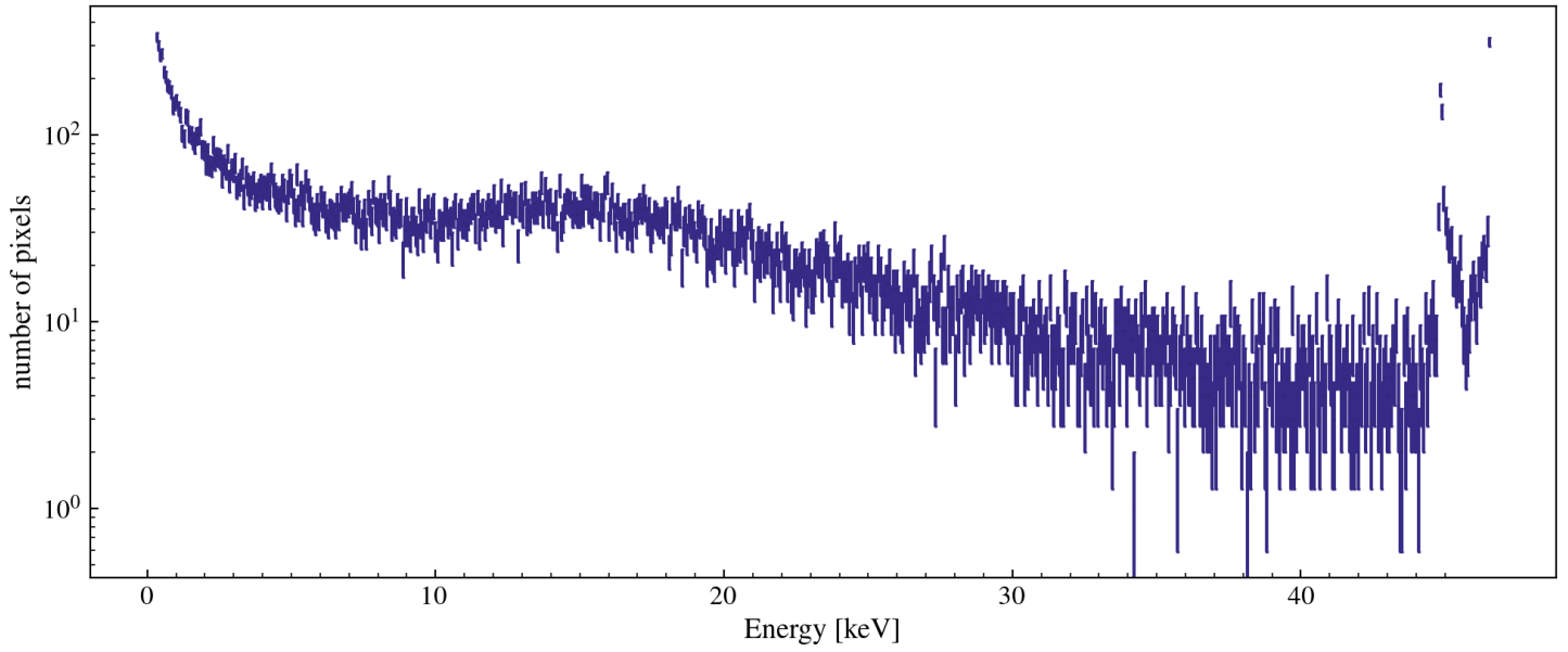
Single Pixel Energy Distribution [w/ 5.18 ADC/e- and 3.74eV/e-] [class MESinglePED]
