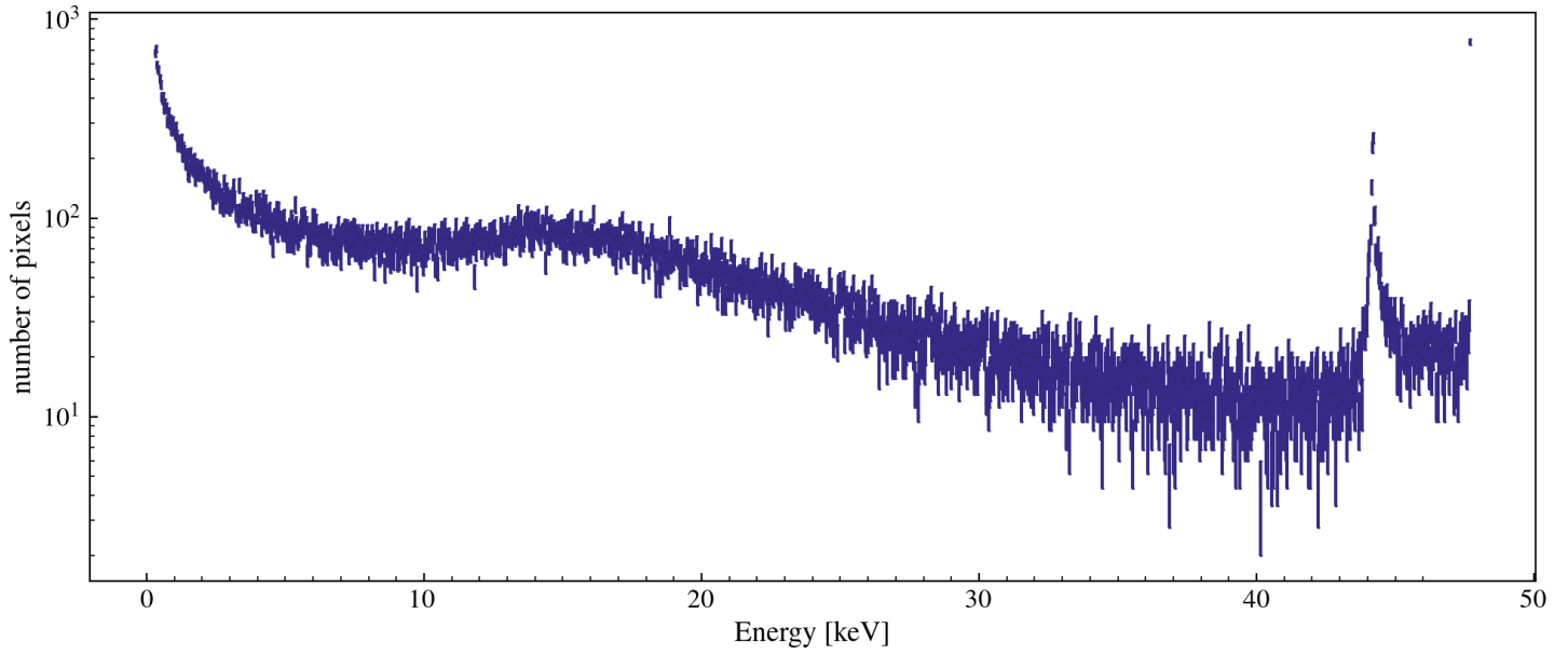
Single Pixel Energy Distribution [w/ 5.05 ADC/e- and 3.74eV/e-] [class MESinglePED]
