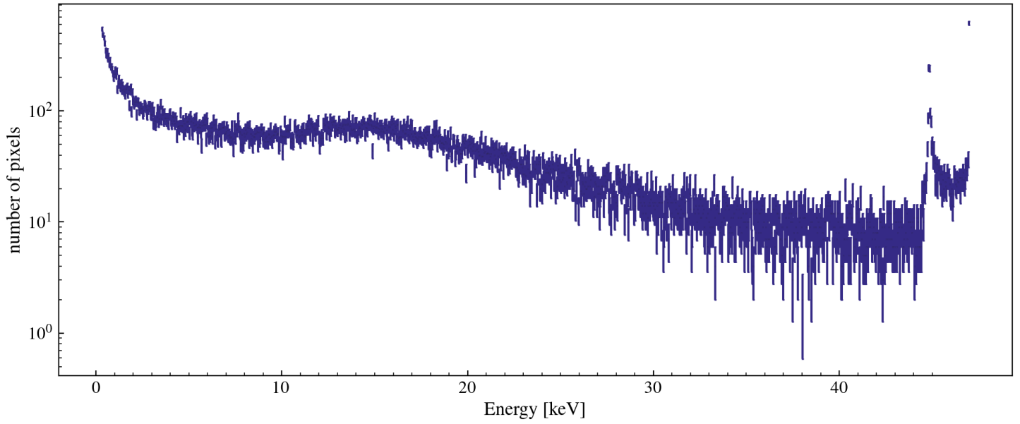
Single Pixel Energy Distribution [w/ 5.13 ADC/e- and 3.74eV/e-] [class MESinglePED]
