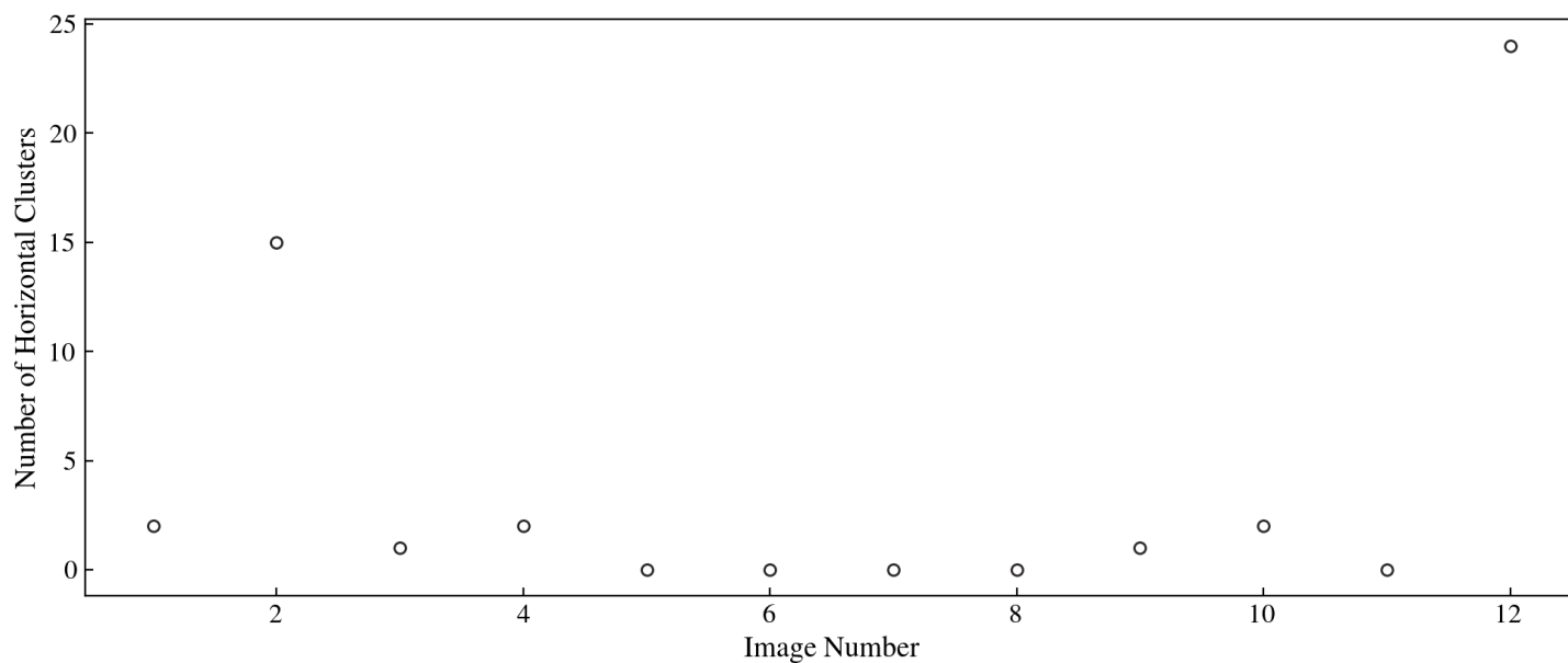
Overscan. Horizontal Clusters vs Image [class MEHorizontalClusters]
