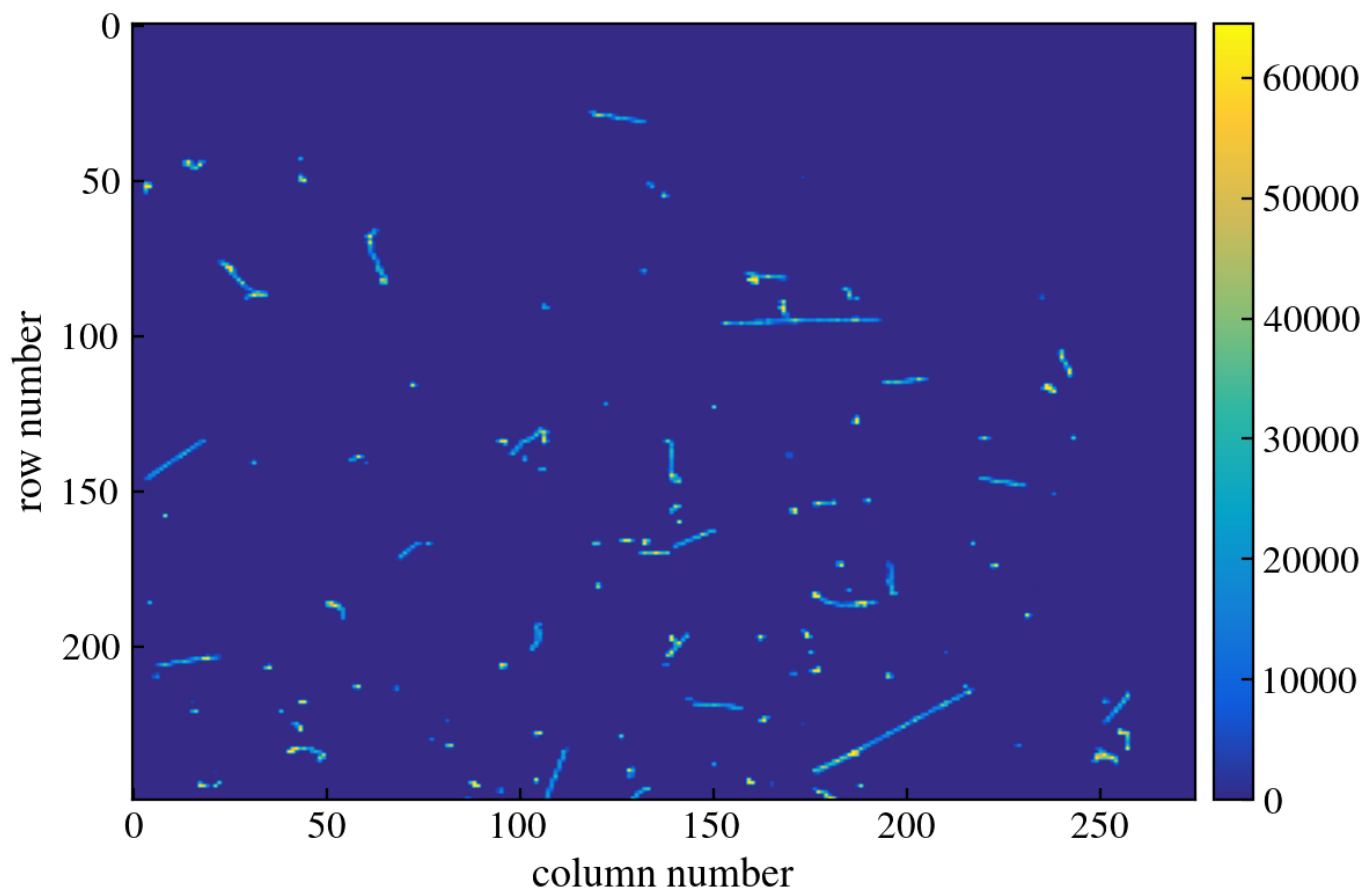
Figure 37: CCD Image
