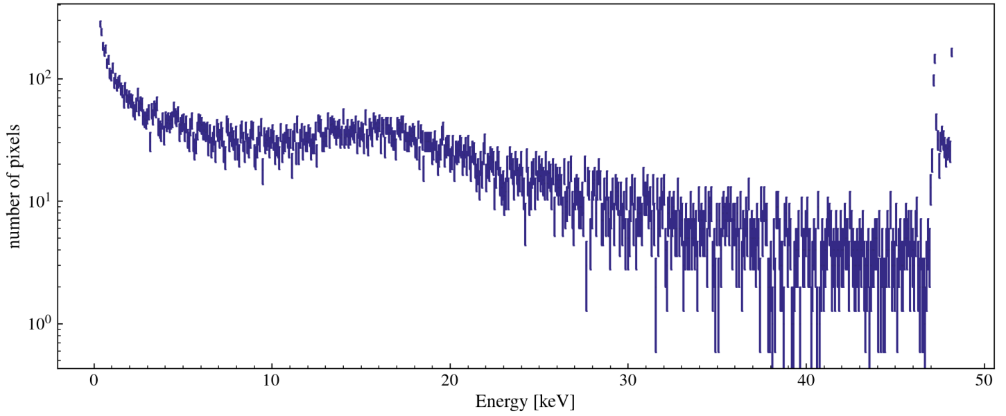
Single Pixel Energy Distribution [w/ 5.0 ADC/e- and 3.74eV/e-] [class MESinglePED]
