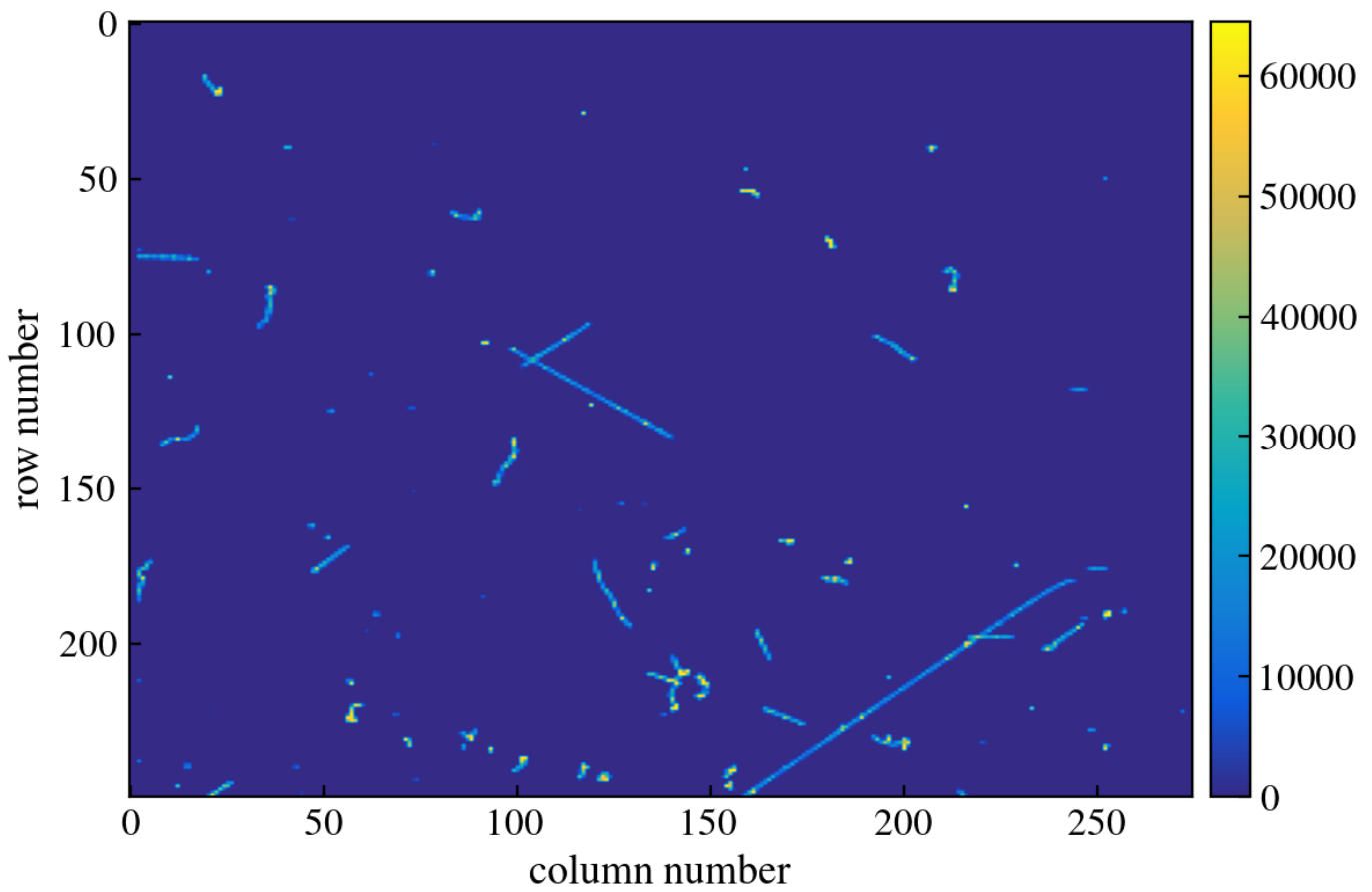
Figure 31: CCD Image
