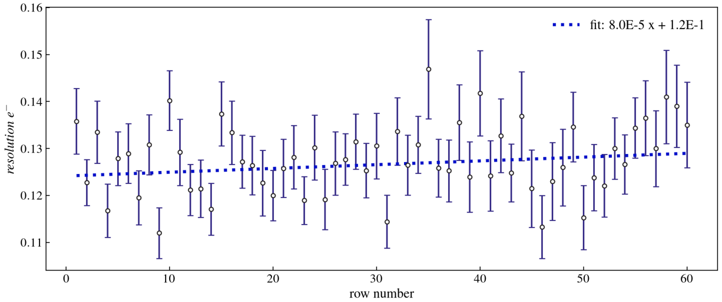
Electron Single Resolution (from MEFitDC per Row) vs row [class MEFitDCSigmaPerRow]
