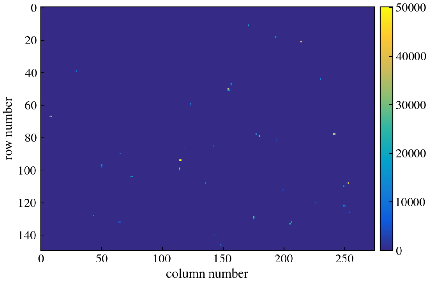
Figure 52: CCD Image
