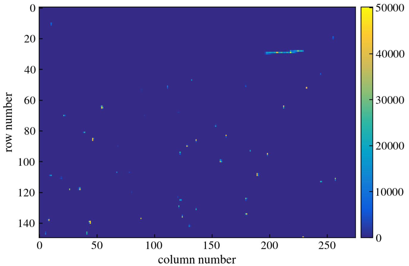
Figure 312: CCD Image
