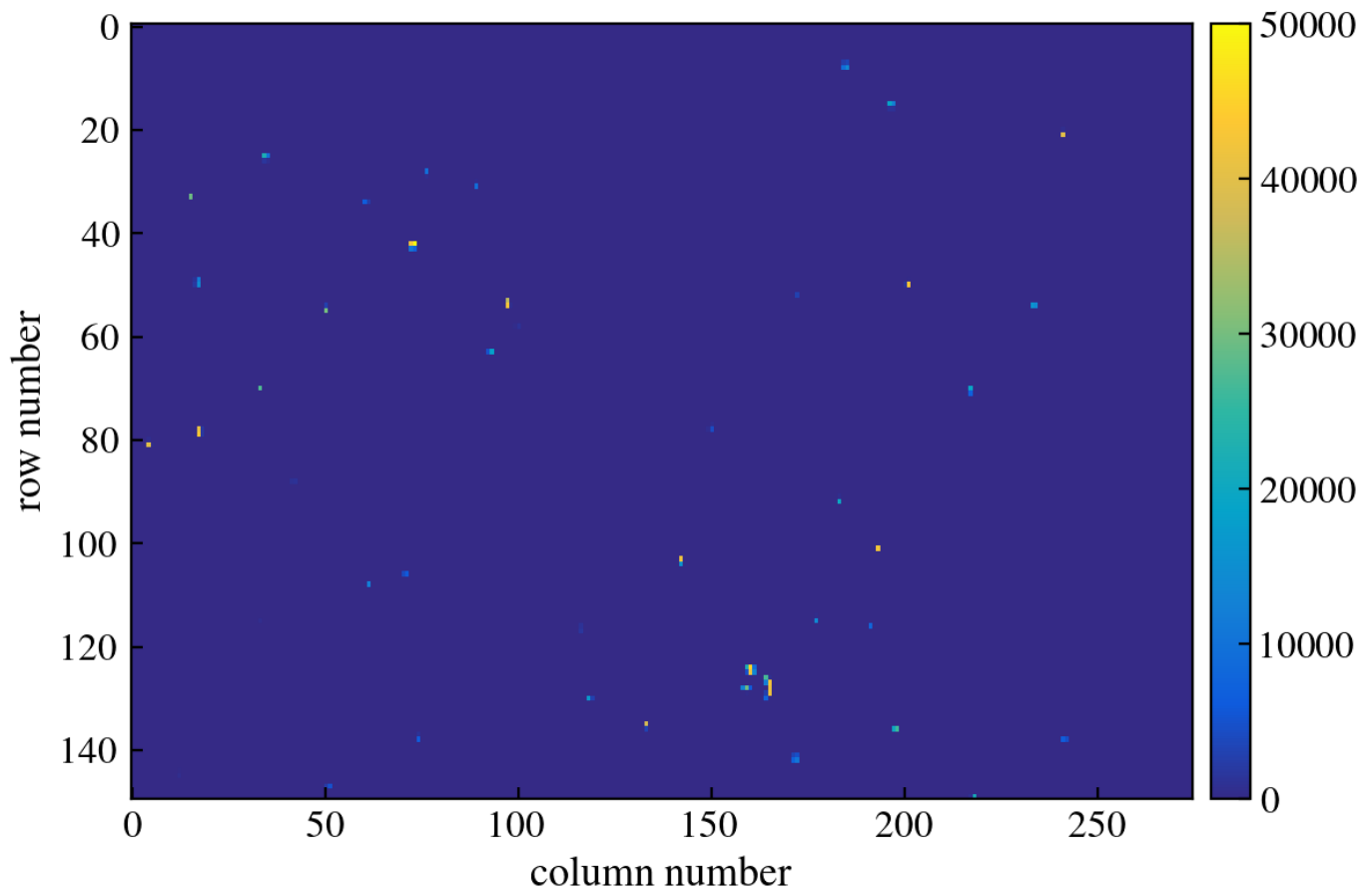
Figure 349: CCD Image
