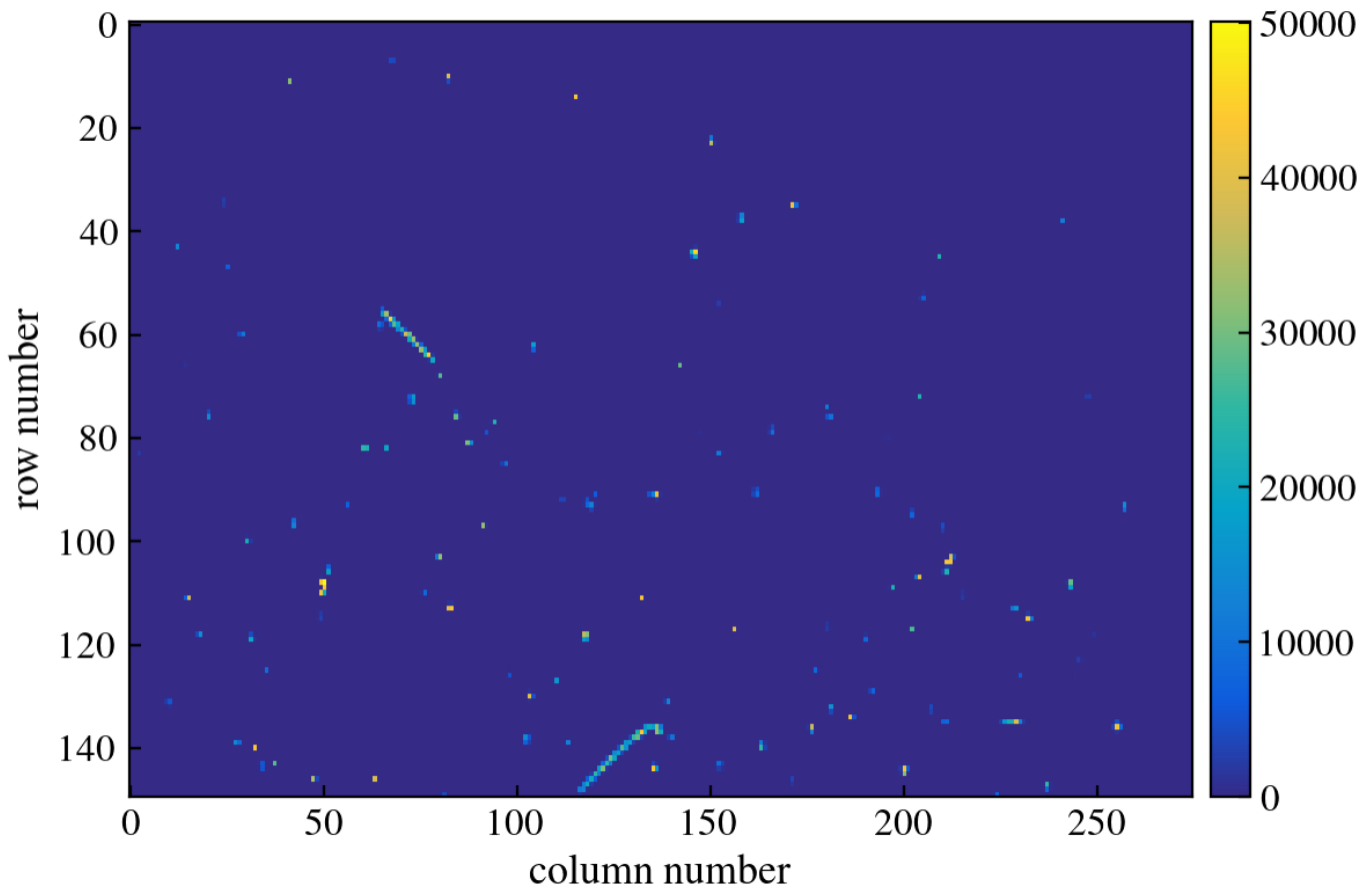
Figure 408: CCD Image
