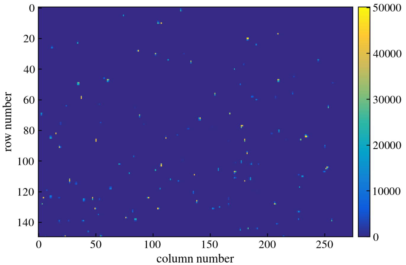
Figure 89: CCD Image
