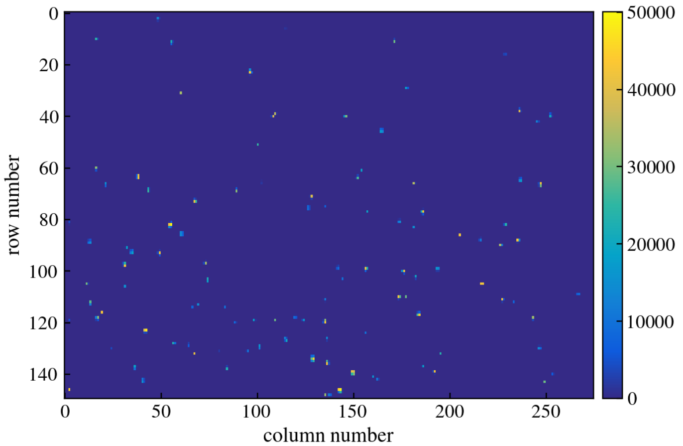
Figure 160: CCD Image
