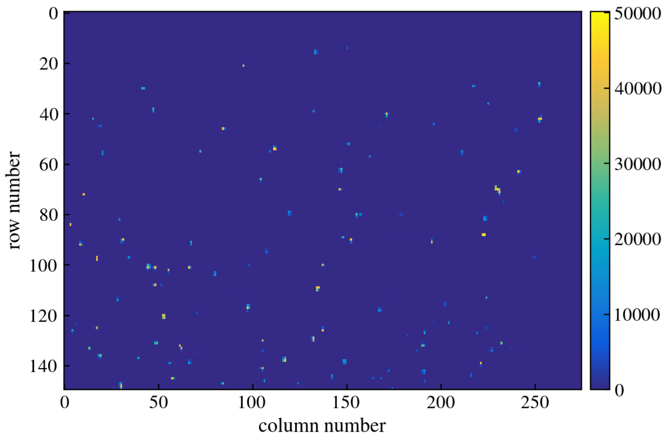
Figure 411: CCD Image
