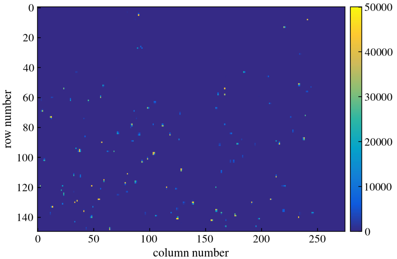
Figure 212: CCD Image
