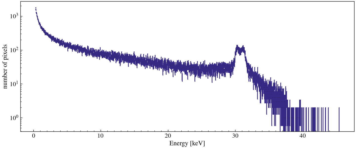
Single Pixel Energy Distribution [w/ 5.24 ADC/e- and 3.77eV/e-] [class MESinglePED]
