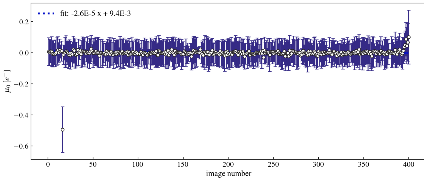
Figure 27: Overscan. PCD Gaussian fit: \mu_0
