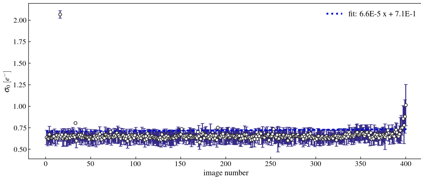
Figure 28: Overscan. PCD Gaussian fit: \sigma_0
