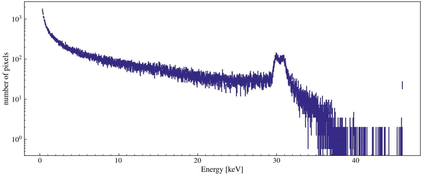
Single Pixel Energy Distribution [w/ 5.29 ADC/e- and 3.77eV/e-] [class MESinglePED]
