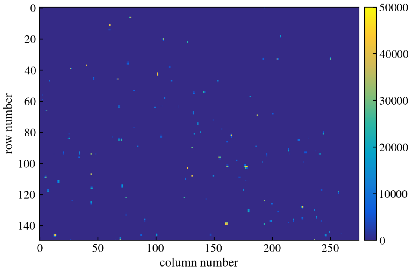
Figure 237: CCD Image
