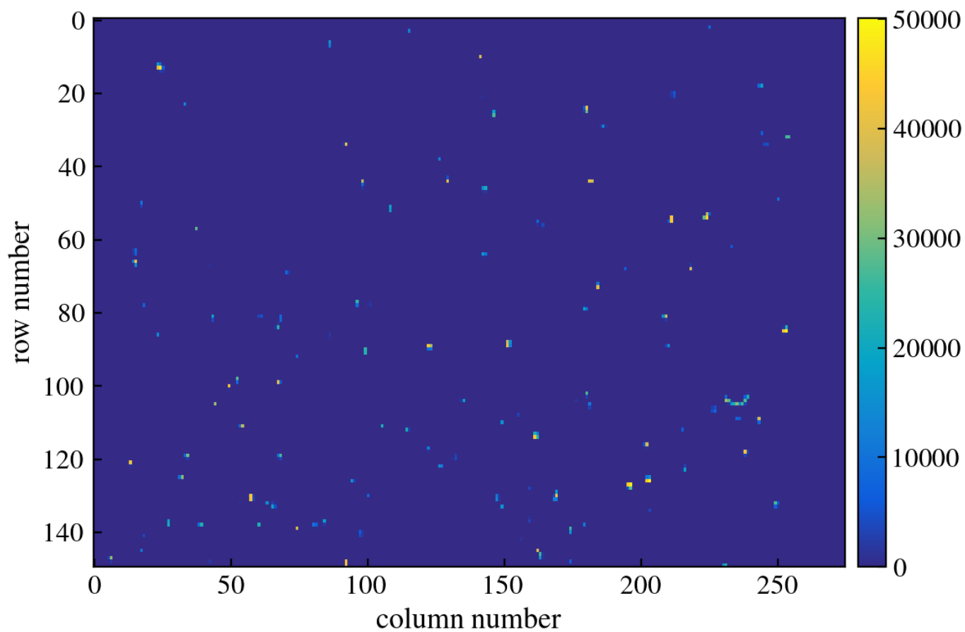
Figure 422: CCD Image
