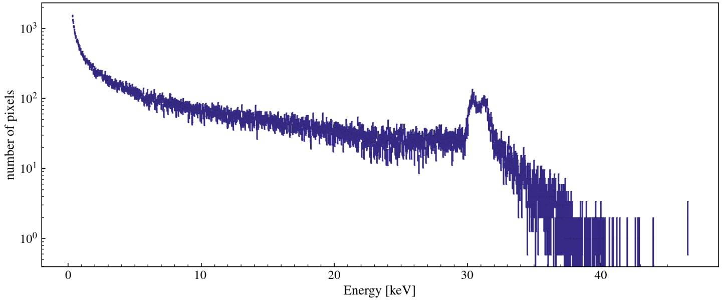
Single Pixel Energy Distribution [w/ 5.22 ADC/e- and 3.77eV/e-] [class MESinglePED]
