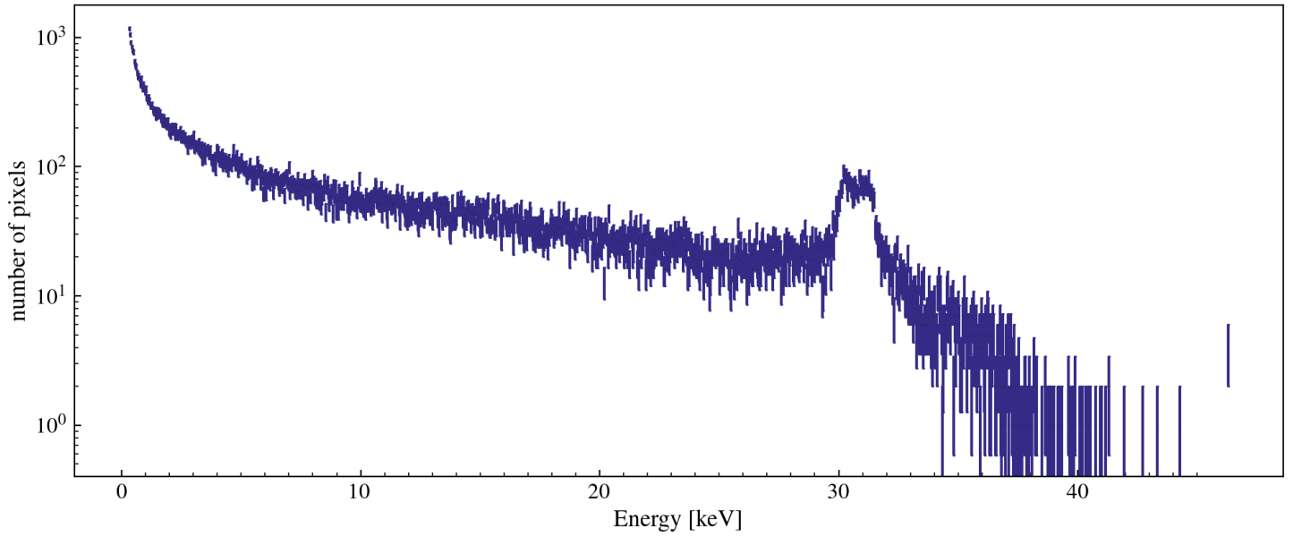
Single Pixel Energy Distribution [w/ 5.25 ADC/e- and 3.77eV/e-] [class MESinglePED]
