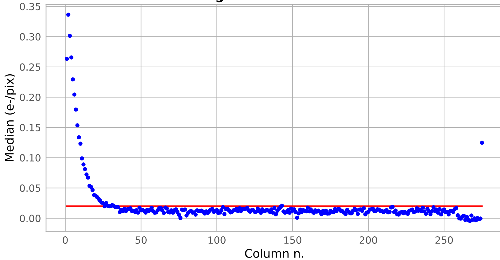
Average dark current vs col
