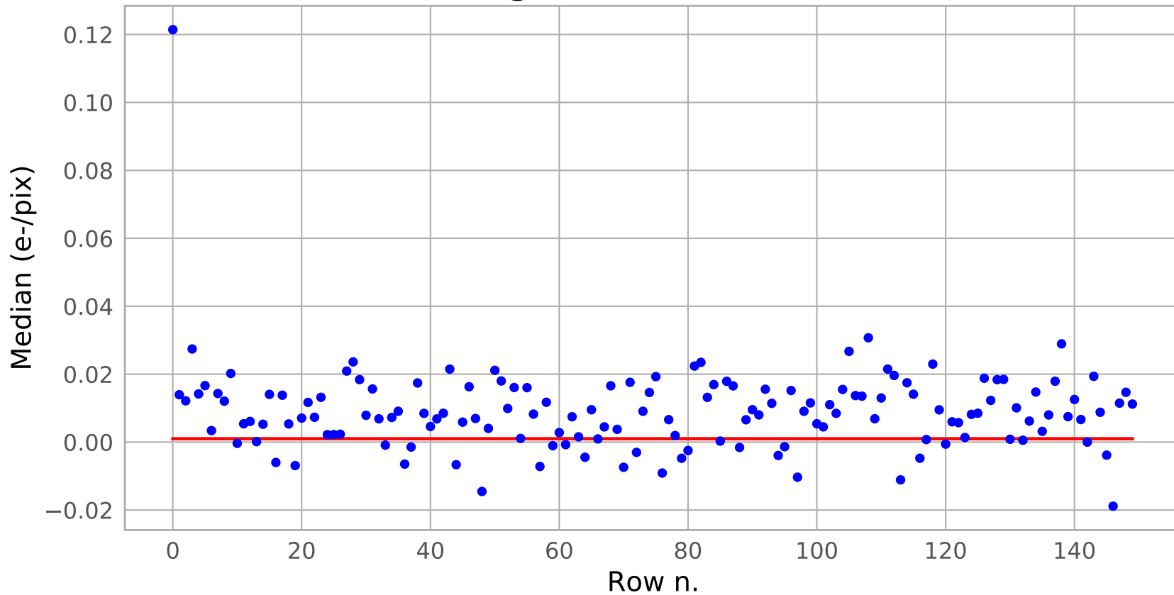
Average dark current vs row
