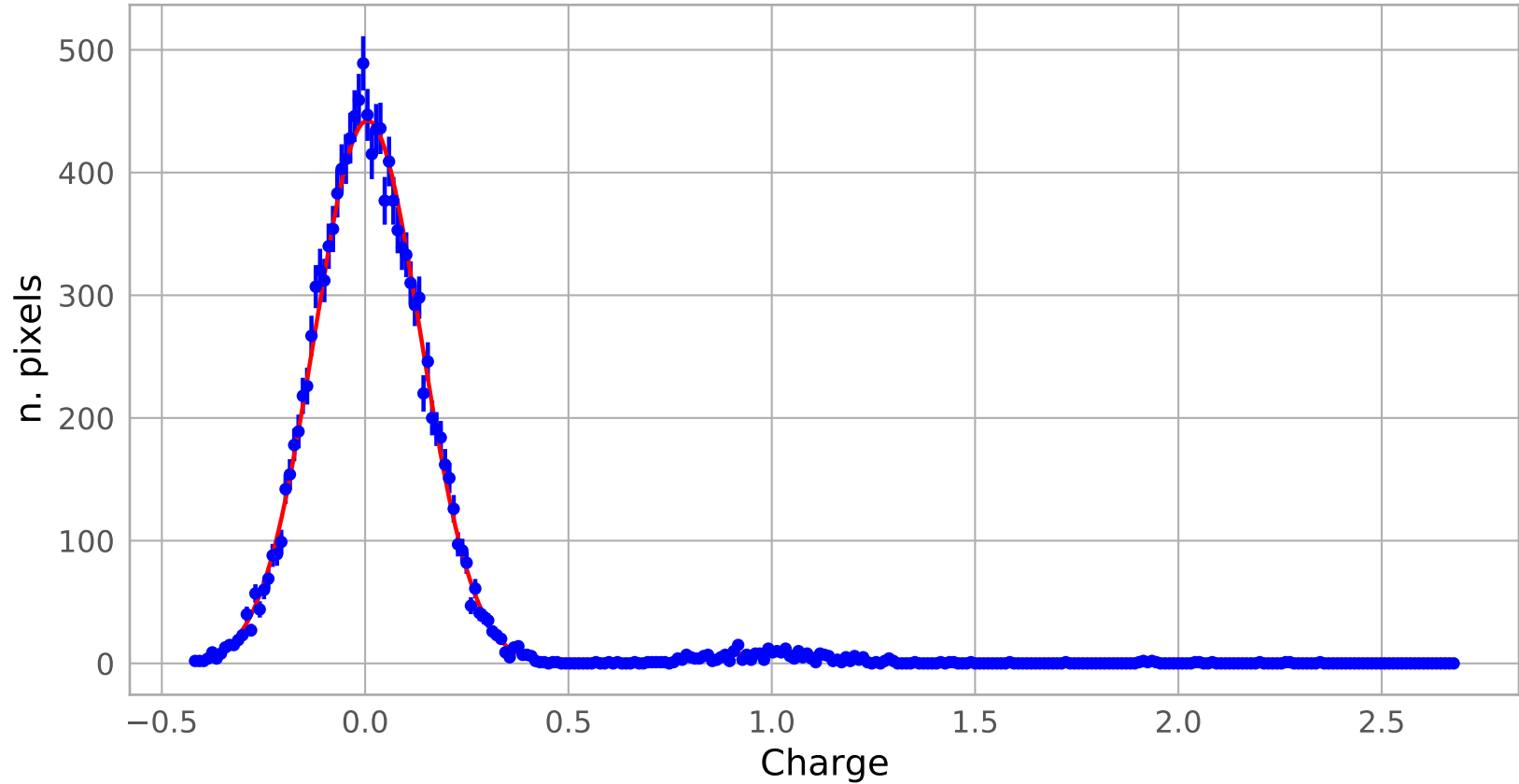
Pixel charge distribution (in e)
