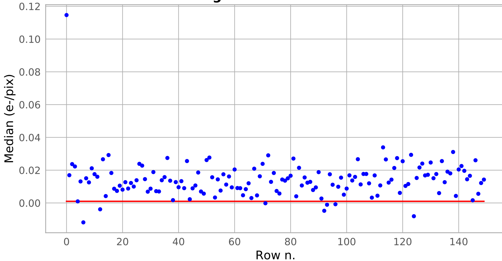
Average dark current vs row
