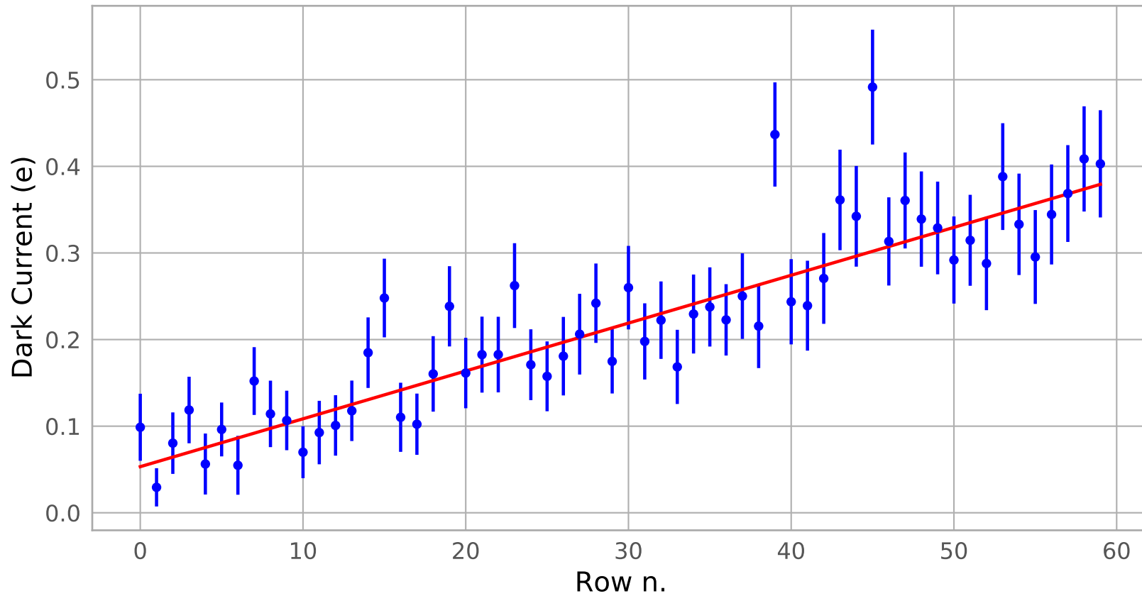
Dark current vs row
