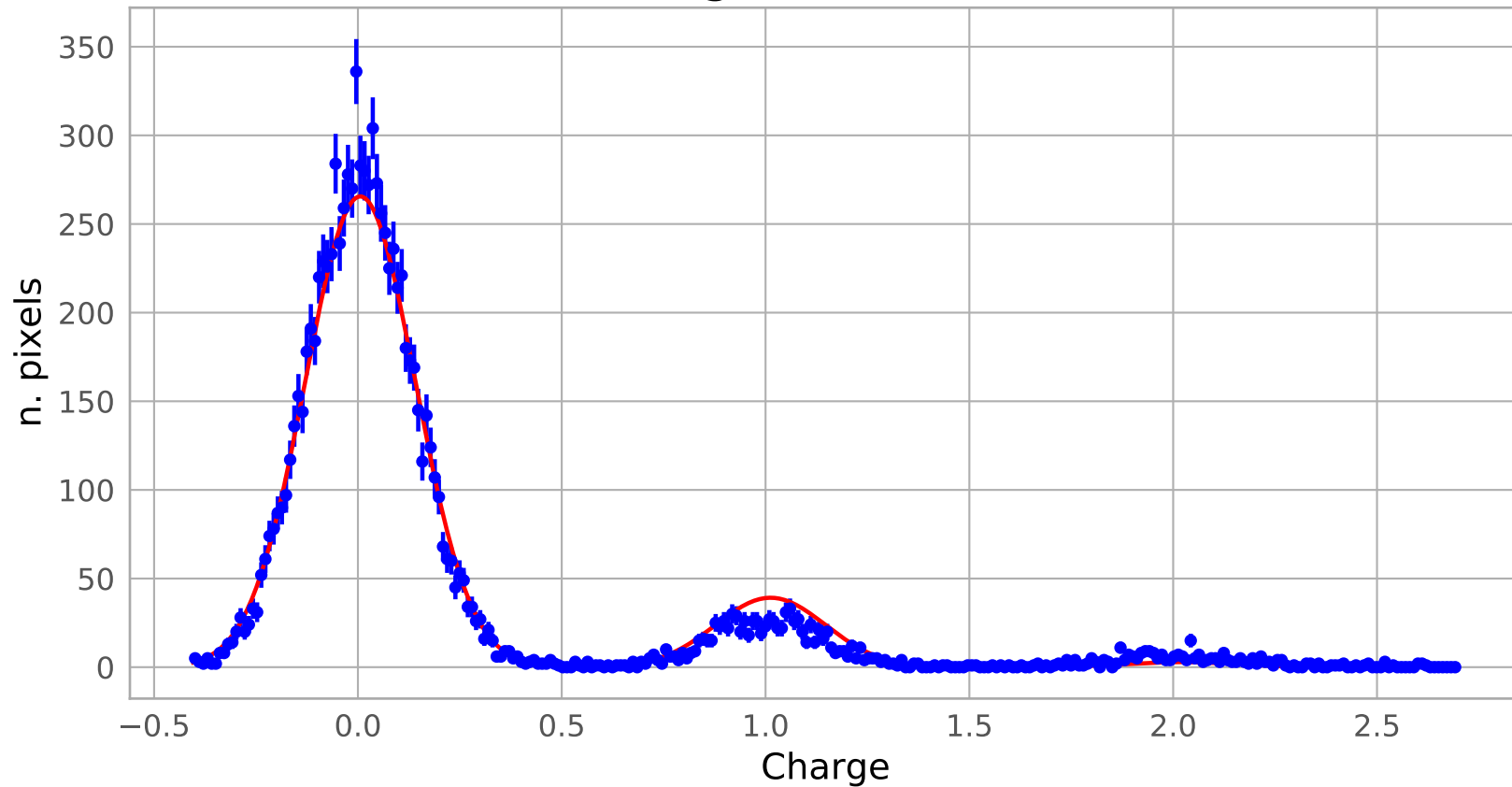
Pixel charge distribution (in e)
