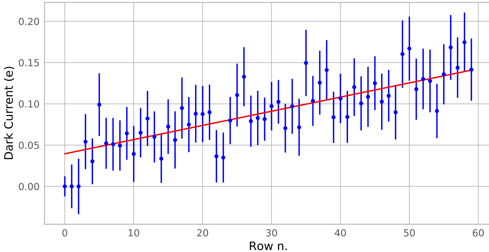
Dark current vs row
