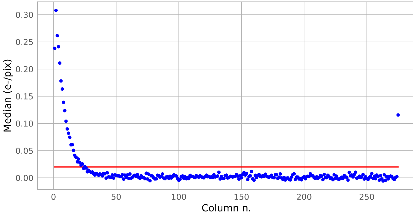
Average dark current vs col
