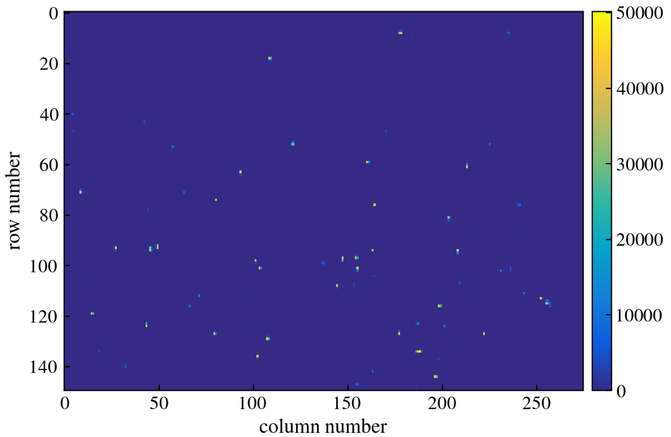
Figure 163: CCD Image
