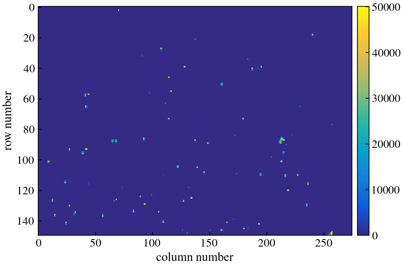
Figure 330: CCD Image
