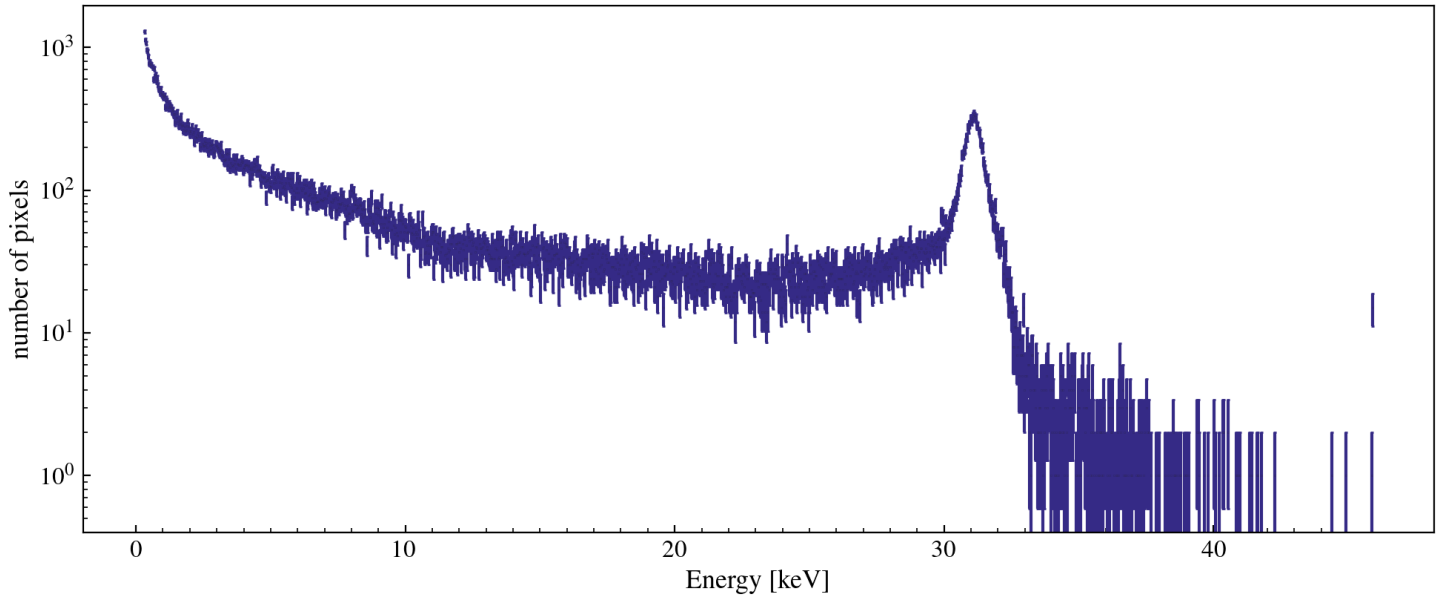
Single Pixel Energy Distribution [w/ 5.25 ADC/e- and 3.74eV/e-] [class MESinglePED]
