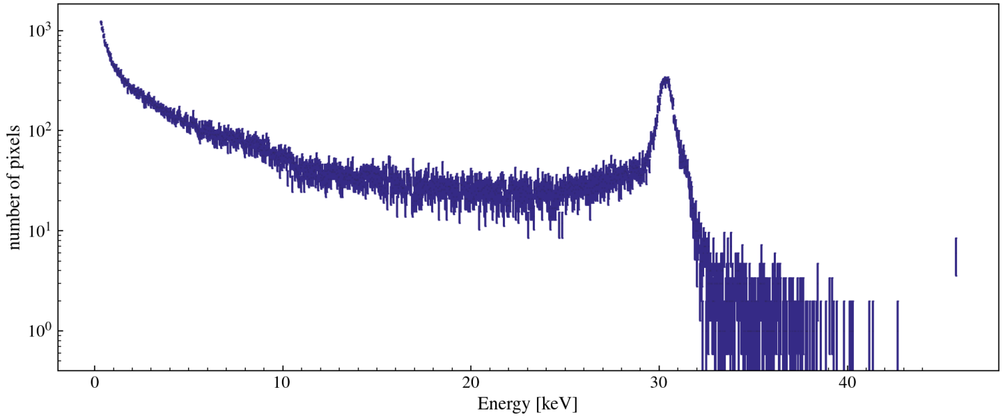
Single Pixel Energy Distribution [w/ 5.26 ADC/e- and 3.74eV/e-] [class MESinglePED]
