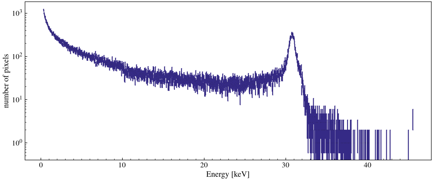
Single Pixel Energy Distribution [w/ 5.29 ADC/e- and 3.74eV/e-] [class MESinglePED]
