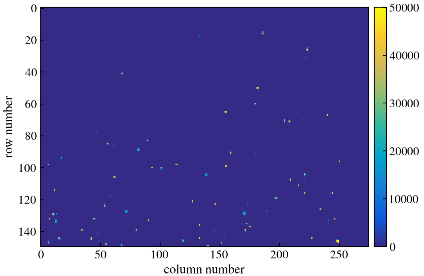
Figure 284: CCD Image
