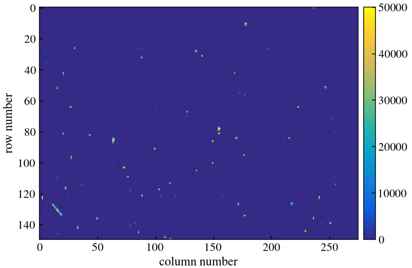
Figure 338: CCD Image
