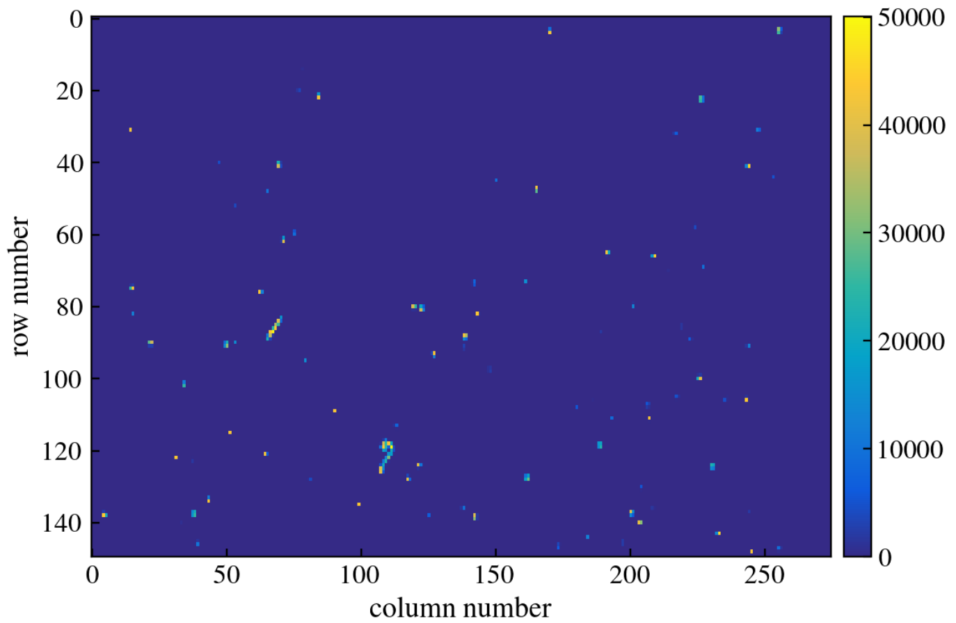
Figure 100: CCD Image
