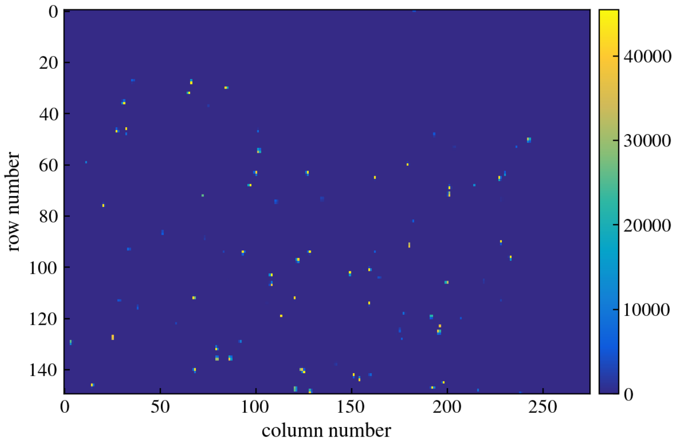
Figure 258: CCD Image
