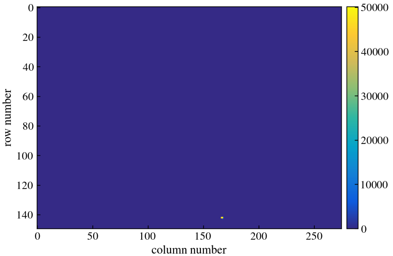
Figure 121: CCD Image
