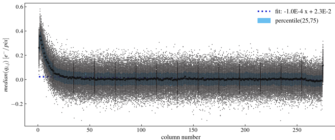
Figure 6: Full Image. Baseline vs column
