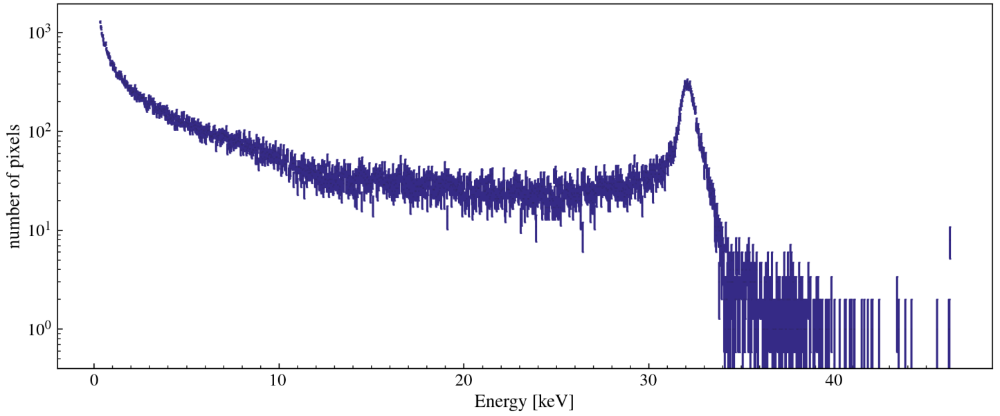
Single Pixel Energy Distribution [w/ 5.21 ADC/e- and 3.74eV/e-] [class MESinglePED]
