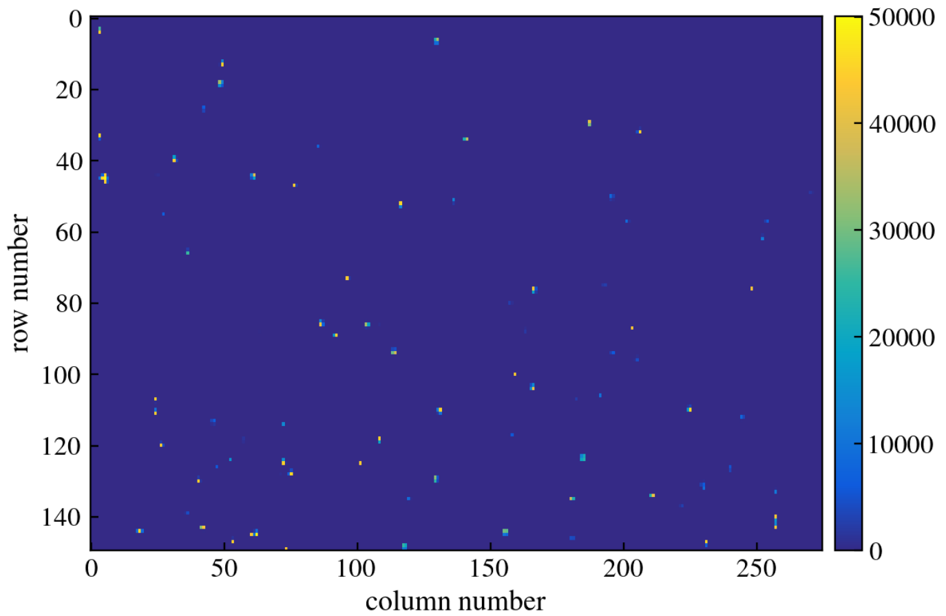
Figure 127: CCD Image
