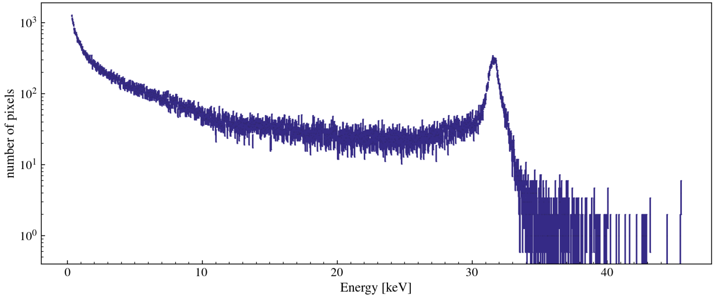
Single Pixel Energy Distribution [w/ 5.3 ADC/e- and 3.74eV/e-] [class MESinglePED]
